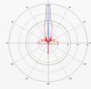
Vertical polarization
