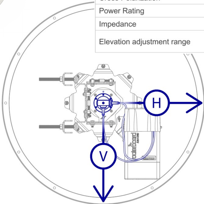
Horizontal/Vertical polarization*
