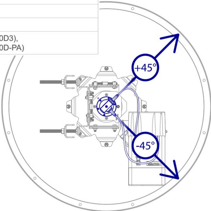
+45°/-45° polarization*
